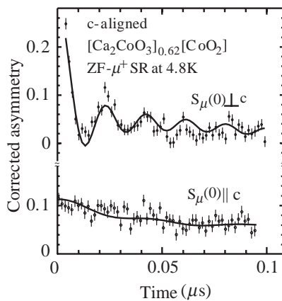
Fig. 6 ZF- \mu^+ SR time spectra of the c -aligned [\text{Ca}_2\text{CoO}_3]_{0.62}^{\text{RS}}[\text{CoO}_2] plate at 4.8 K. The configurations of the sample and the initial muon spin direction \mathbf{S}_{\mu}(0) are (top) \mathbf{S}_{\mu}(0) \perp c and (bottom) \mathbf{S}_{\mu}(0) \parallel c .
