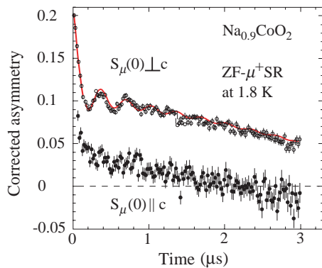
Fig. 2 ZF- \mu^+ SR time spectra of single crystal platelets of Na 0.9 CoO 2 at 1.8 K. The configurations of the sample and the initial muon spin direction S_\mu(0) are (top) S_\mu(0) \perp c and (bottom) S_\mu(0) \parallel c . The bottom spectrum is offset below to be seen clearly.
