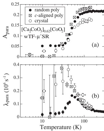
Fig. 5 (a) Paramagnetic \mu^+ spin precession asymmetry A_{\text{para}} and (b) muon spin relaxation rate \lambda_{\text{para}} as a function of temperature for the three [\text{Ca}_2\text{CoO}_3]_{0.62}^{\text{RS}}[\text{CoO}_2] samples: a randomly oriented polycrystalline disk (solid circles), 12) a c -axis aligned polycrystalline plate (squares) and single crystal (SC) platelets (open circles). For the SC platelets, both the value of A_{\text{para}} above 100 K and the change in A_{\text{para}} below 100 K are smaller than those in the polycrystalline samples. This is because the muon momentum was decreased from 28 to 25 MeV/c for the SC measurements to stop muons in the thin platelets ( \sim 100 \mu\text{m} thickness), causing a small background signal from muons stopping elsewhere.
