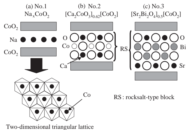
Fig. 1 Schematic crystal structures of layered cobaltites; (a) \text{Na}_x\text{CoO}_2 , (b) 3-layer cobaltites, and (c) 4-layer cobaltites.
