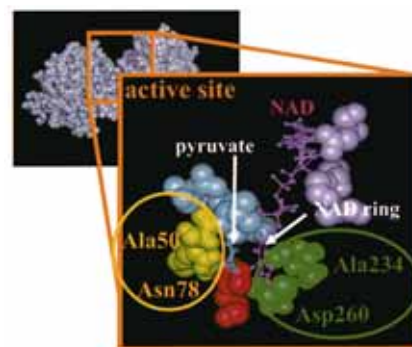
Fig. 2 The structural model of the active site of D-LDH.
