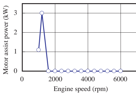
Fig. 12 Motor assist power (two-stage).
