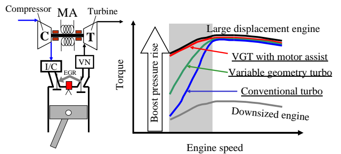
Fig. 3 The means of the low-end torque improvement.
