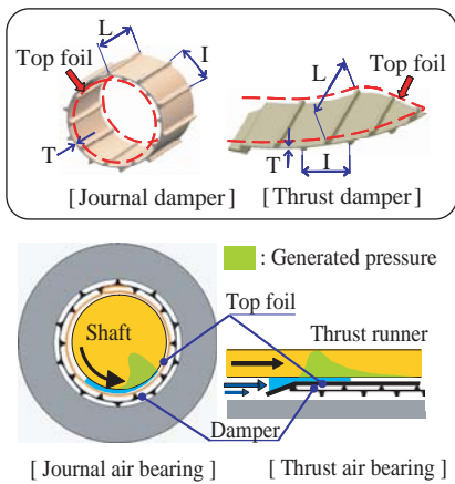
Fig. 1 Compliant foil bearings.
