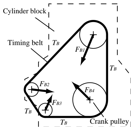
Fig. 8 Belt element.
