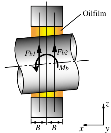
Fig. 6 Journal bearing element (side view).
