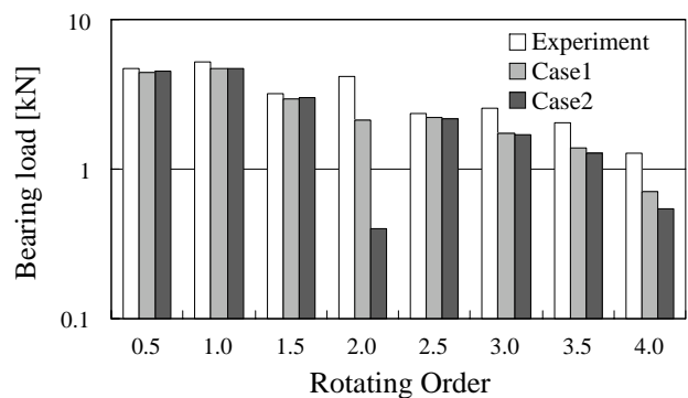
Fig. 13 Spectrum of bearing load. (#1 main bearing, vertical direction)
