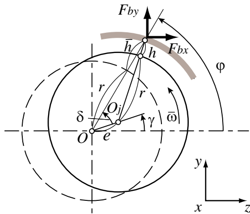
Fig. 5 Journal bearing element (cross section).
