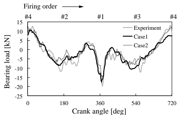
Fig. 12 Bearing load. (#1 main bearing, vertical direction)
