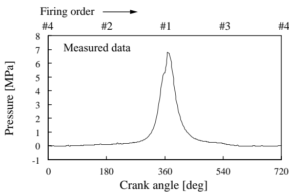
Fig. 10 Cylinder gas pressure (#1 cylinder).
