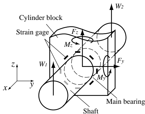
Fig. 11 Measurement of bearing load.
