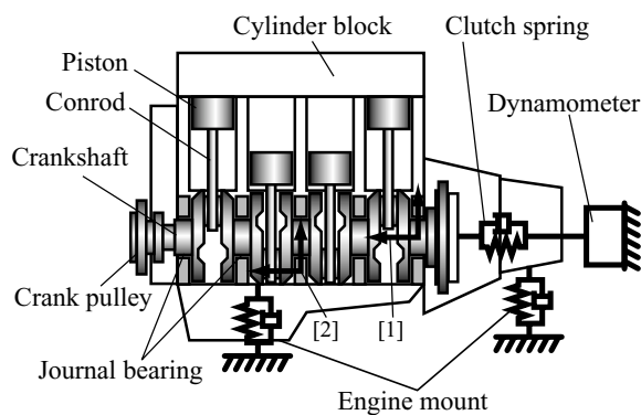
Fig. 2 Model of inline 4-cylinder engine.
