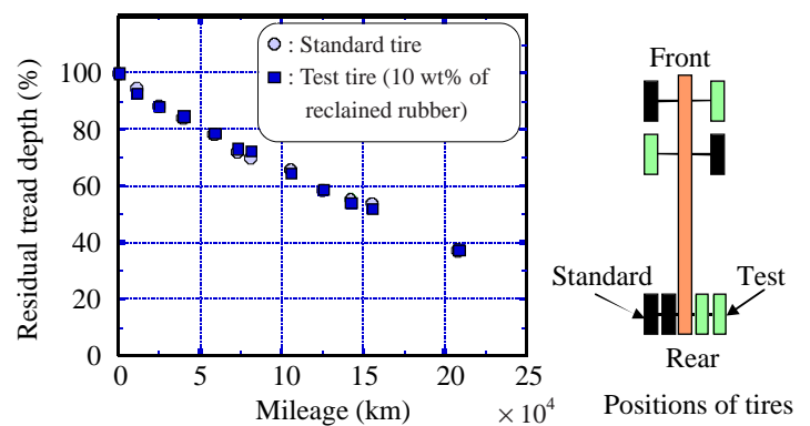
Fig. 11 Changes in tread depth for standard and test truck tires during actual road tests.
