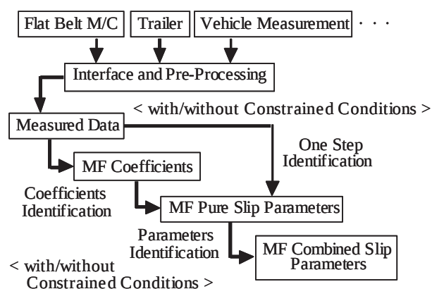
Fig. 1 Structure of tire model identification system.
