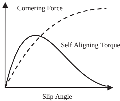
Fig. 8 Relationship between side force and self aligning torque with slip angle.
