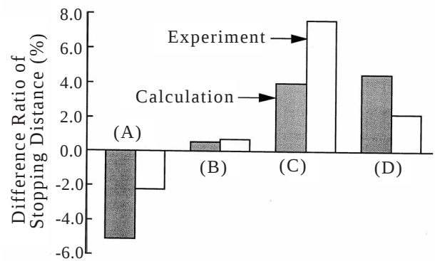
Fig. 5 Comparison of stopping distance between calculation and experiments.
