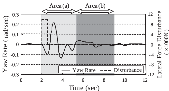
Fig. 11 Time history of yaw rate at corrective steering.
