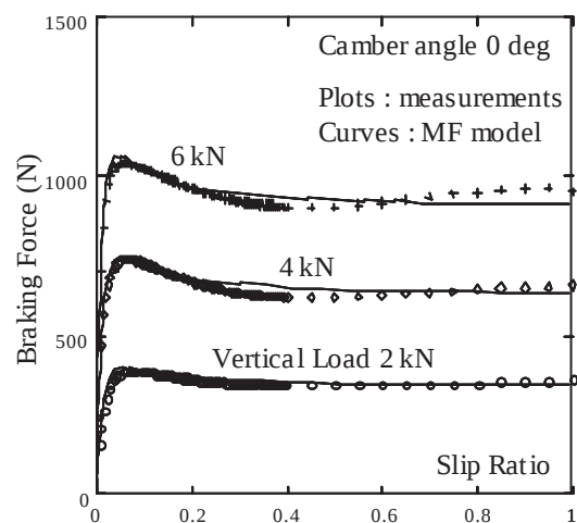
(a) Passenger vehicle tire : 195/65R15
