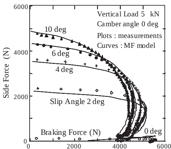
Fig. 2 Combined slip characteristics on dry road (Passenger vehicle tire : 195/65R15).
