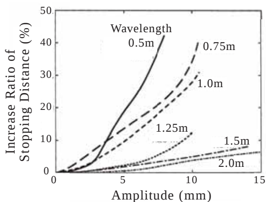
Fig. 6 Influence of wavelengths and amplitudes of road undulations on stopping distance.
