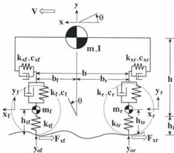
Fig. 4 Vehicle model and symbol notation.
