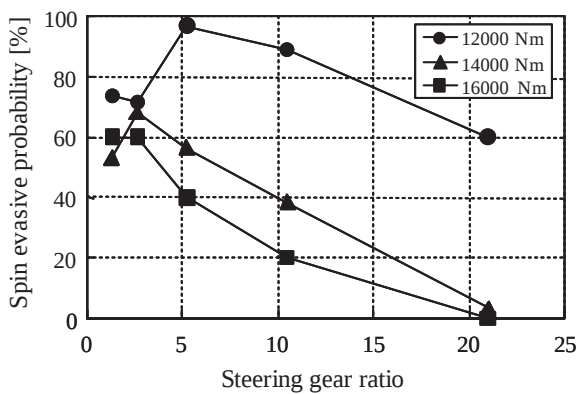
Fig. 10 Spin evasive probability to steering gear ratio and yaw moment disturbance.
