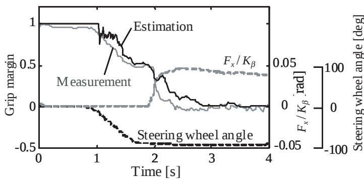
Fig. 9 Comparison of estimated and measured grip margin at combined slip condition.
