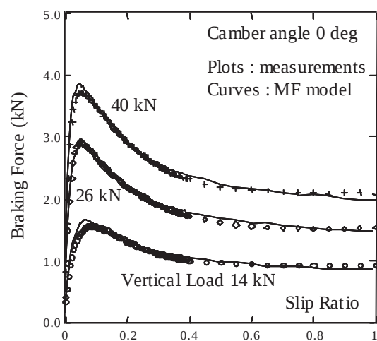
(b) Commercial vehicle tire : 11R22.5
