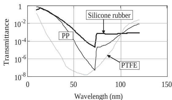
Fig. 1 Calculated absorptions of VUV for polypropylene (PP), silicone rubber and polytetrafluoroethylene (PTFE).
