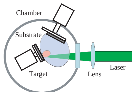
Fig. 2 Schematic setup for the polymer surface treatment with VUV and nanometer-sized particles.
