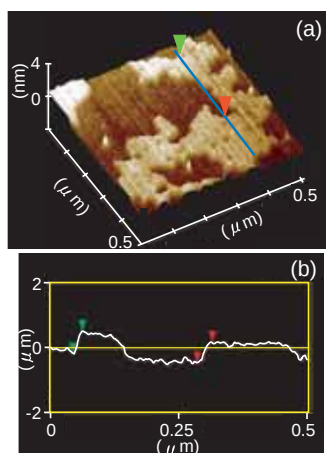
Fig. 1 (a) AFM image of silica nanosheets on a mica surface, and (b) the height profile of image (a).
