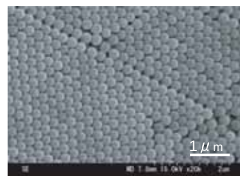
Fig. 2 SEM image of a three-dimensional crystal of silicon-coated colloidal silica.
