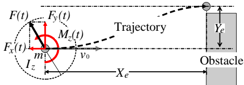
Fig. 4 Collision avoidance problem for a rigid body.
