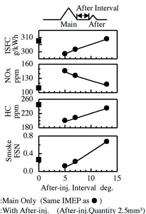
Fig. 8 Effect of after-injection interval on emissions (End of main to start of after).
