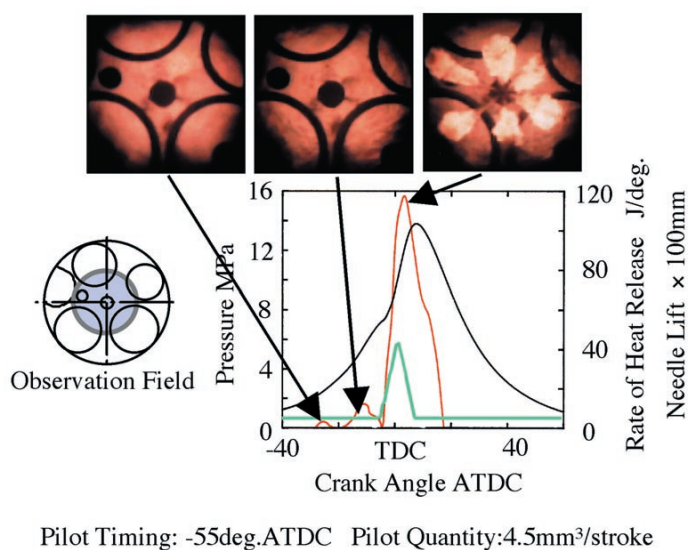
Fig. 2 Combustion process of early-pilot injection at full load.
