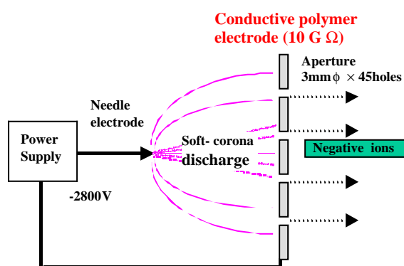
Fig. 1 Structure of negative ion generator.
