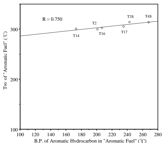
Fig. 7 Boiling point of aromatic hydrocarbon in "Aromatic Fuels" and T_{90} of "Aromatic Fuels".
