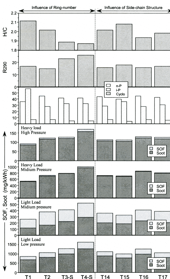
Fig. 11 Fuel properties and SOF and soot emissions from "Aromatic Fuels".
