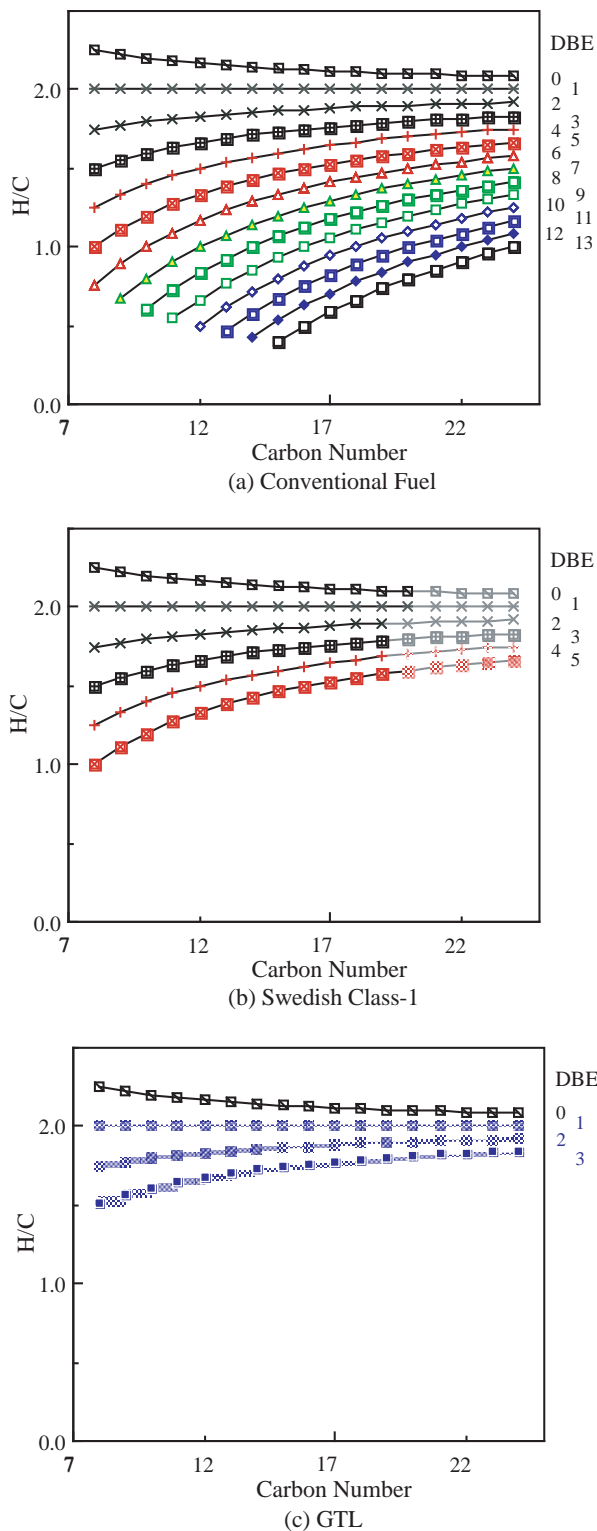
Fig. 14 Compositions of conventional fuel, swedish Class-1 and GTL.
