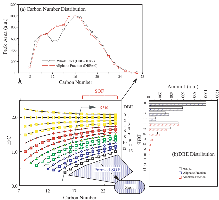
Fig. 1 Precise analytical results of diesel fuel and PM formation.
