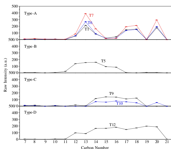
Fig. 4 Carbon number distributions of n-paraffins in "Aliphatic Fuels".
