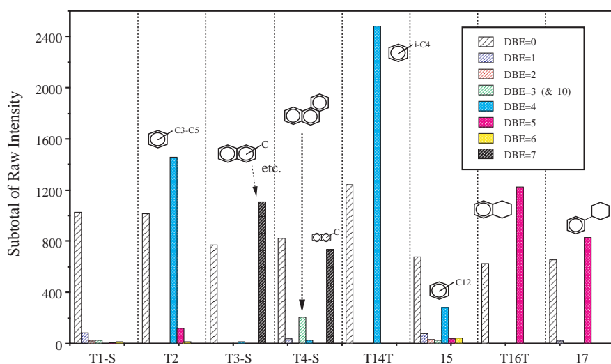
Fig. 3 DBE distributions of "Aromatic Fuels".
