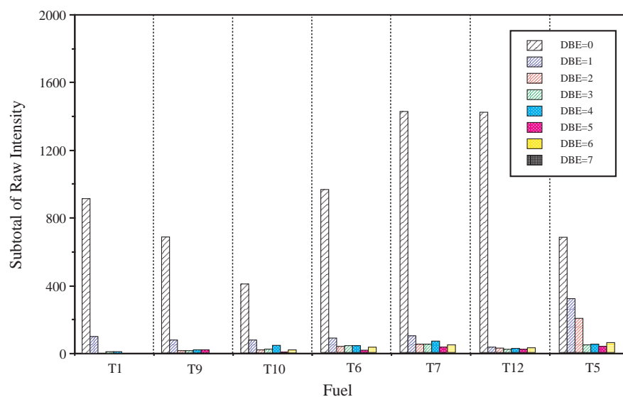
Fig. 2 DBE distributions of "Aliphatic Fuels".
