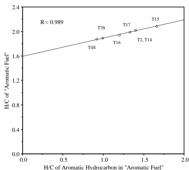
Fig. 8 H/C of aromatic hydrocarbon in "Aromatic Fuels" and H/C of "Aromatic Fuels".
