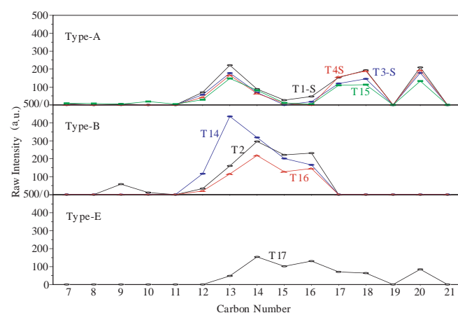
Fig. 5 Carbon number distributions of n-paraffins in "Aromatic Fuels".
