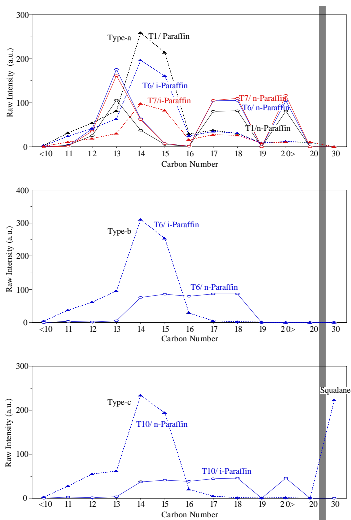
Fig. 6 Carbon number distributions of i-paraffins in "Aliphatic Fuels".
