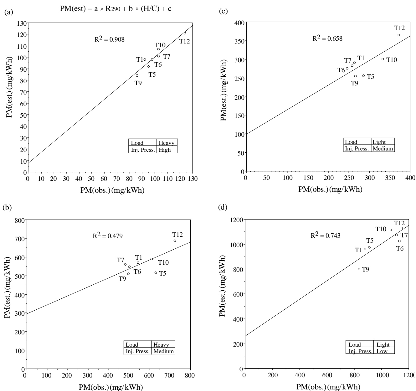
Fig. 12 PM emissions observed and estimated from "Aliphatic Fuels".
