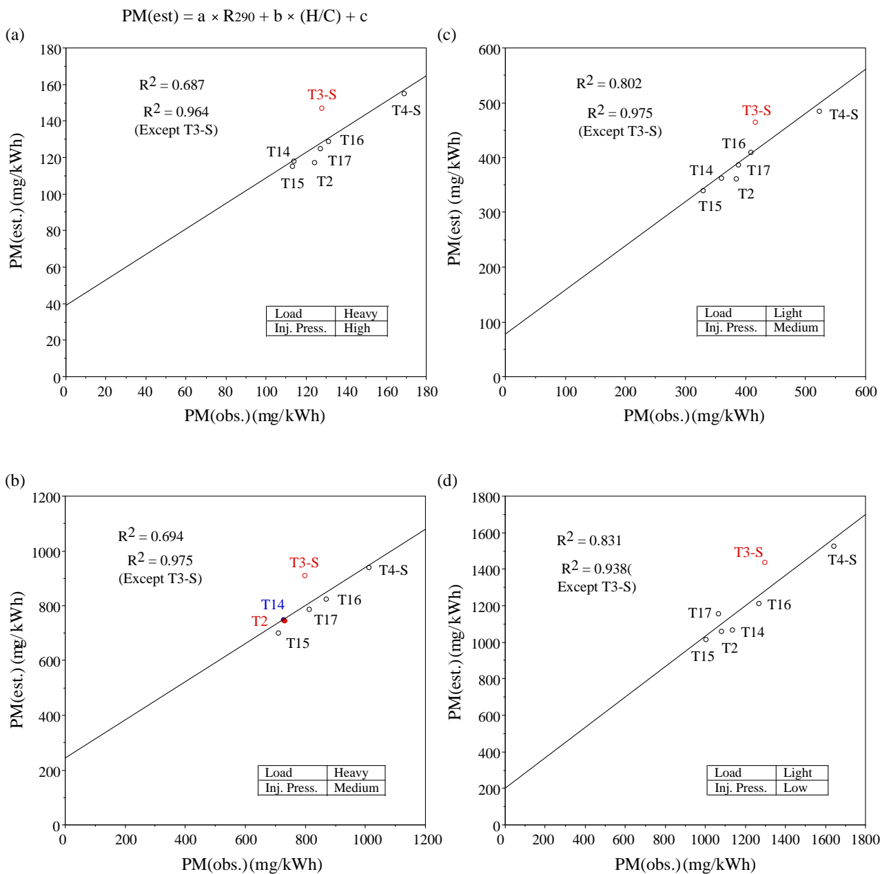
Fig. 13 PM Emissions Observed and Estimated from "Aromatic Fuels".
