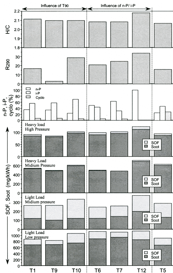
Fig. 10 Fuel properties and SOF and soot emissions from "Aliphatic Fuels".
