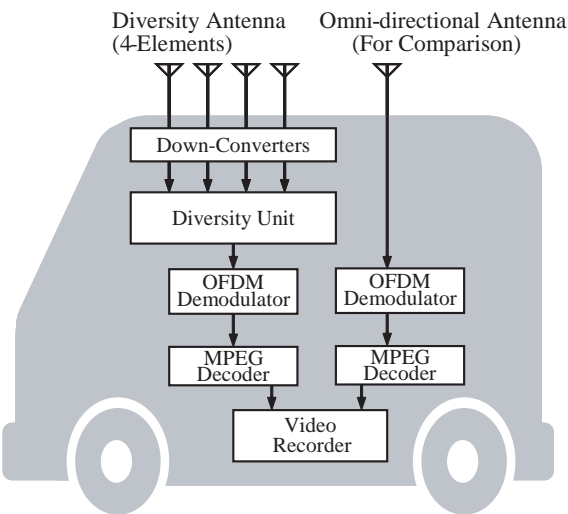
Fig. 2 Outline of experimental setup.
