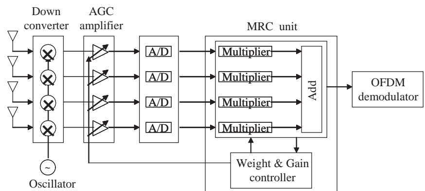
Fig. 1 Block diagram of the receiver system.
