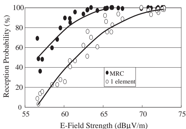
Fig. 7 Relation between the reception probability and the electric field strength.
