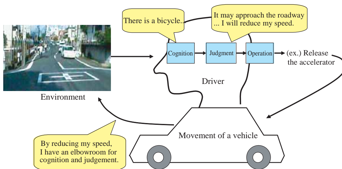
Fig. 1 Block diagram of a vehicle regarded as a human-machine cooperative system.
