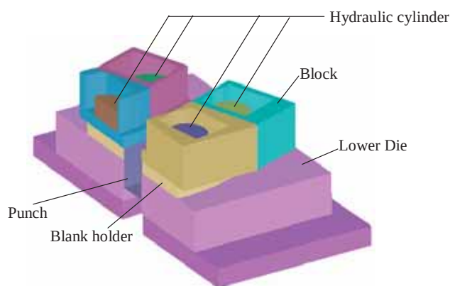
Fig. 6 Modeling of elastic die.
