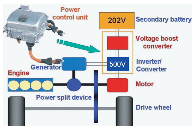
Fig. 5 Schematic view of THS II system of Prius. The power control unit contains an inverter and a DC/DC converter. In THS II, a high-voltage power circuit that increases the voltage up to 500V is added.
