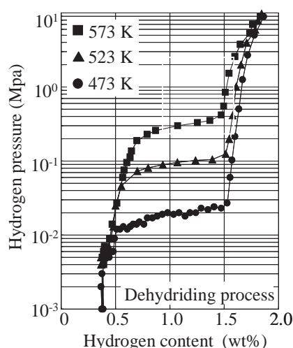
Fig. 2 The p - c isotherms of CaSi in dehydrogenating processes at 473 K, 523 K and 573 K.
