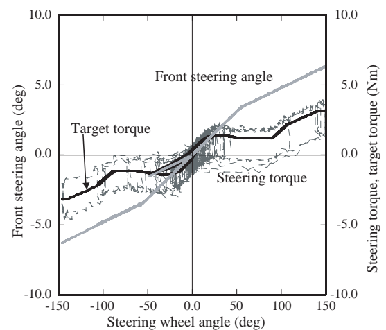
Fig. 4 Front steering angle and steering torque for drift-out test.
