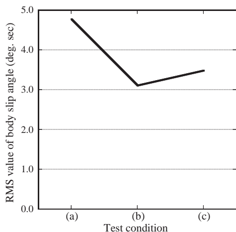
Fig. 8 RMS values of body slip angle at spin test.
