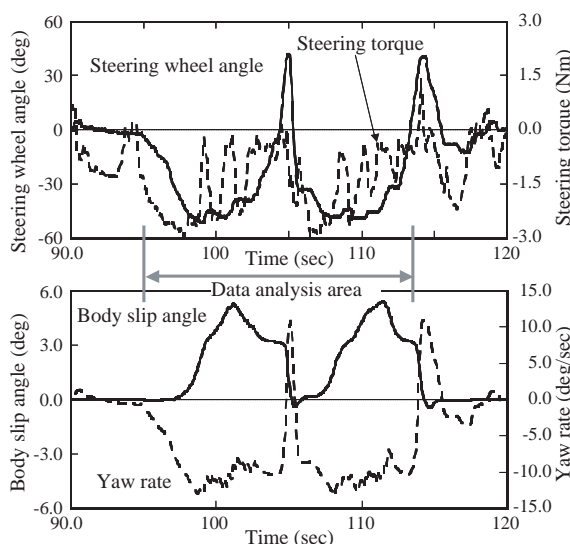
Fig. 7 Time histories of spin test.
