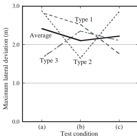
Fig. 5 Maximum lateral deviation for drift-out test.
