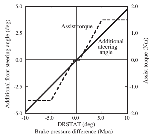
Fig. 6 Additional front steering angle and assist steering torque for spin test.
