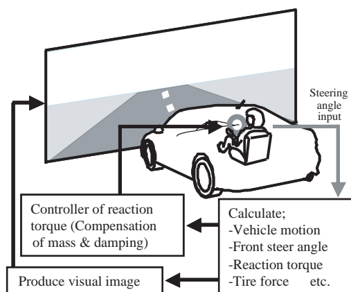
Fig. 1 Configuration of driving simulator.
