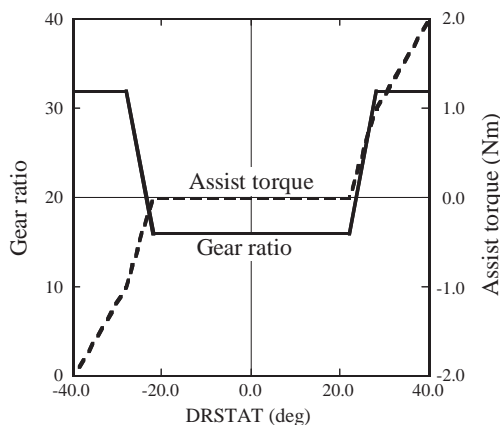
Fig. 3 Gear ratio and assist steering torque for drift-out test.
