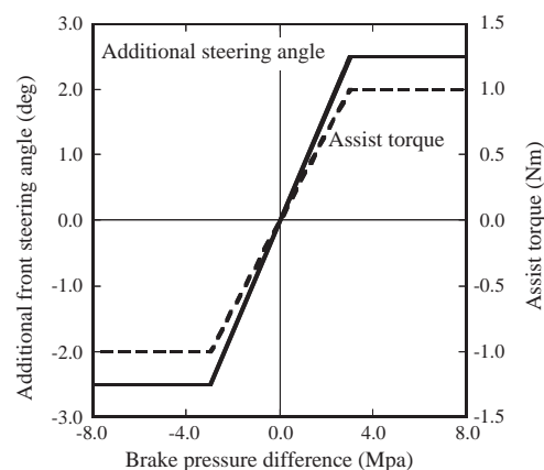
Fig. 9 Additional front steering angle and assist steering torque for split \mu braking test.
