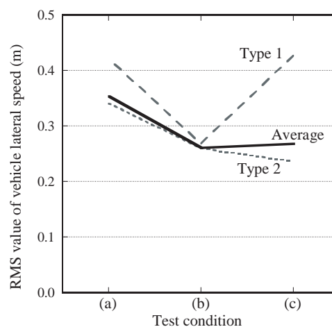
Fig. 10 RMS values of vehicle lateral speed for split \mu braking test.
