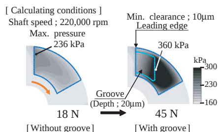
Fig. 3 Comparison of load capacity (calculated).
