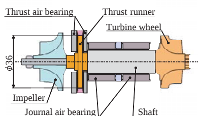
Fig. 2 Construction of air bearings for turbocharger.
