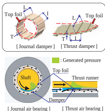
Fig. 1 Compliant foil bearings.
