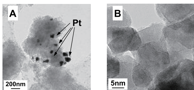
Fig. 4 TEM images of Pt supported catalysts after ageing at 800°C in air for 5 h. (A) Pt/alumina, (B) Pt/CZY (CeO 2 (50wt%)-ZrO 2 (46wt%)-Y 2 O 3 (4wt%)). (19)
