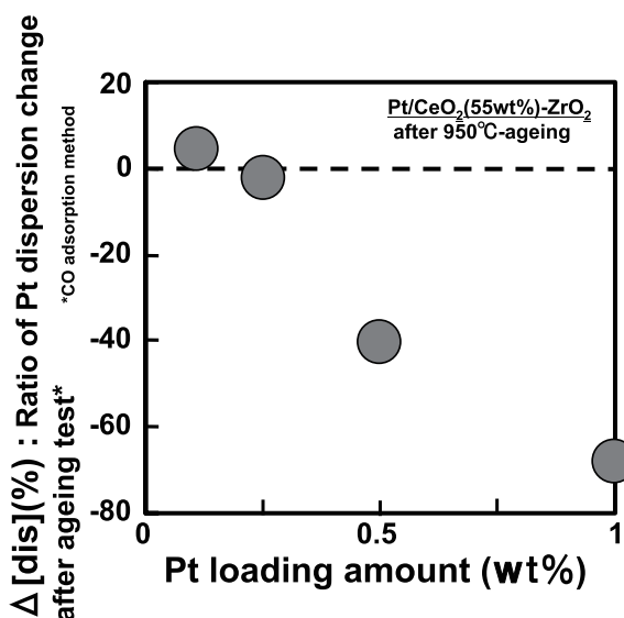
Fig. 12 Effect of Pt loading amount for sintering suppression. Pt loaded ceria-based oxide was aged at 950^\circ\text{C} for 5 h in a simulated exhaust gas. Pt dispersion was measured by the CO pulse adsorption method after an oxidation-reduction pretreatment at 800^\circ\text{C} . (26)
