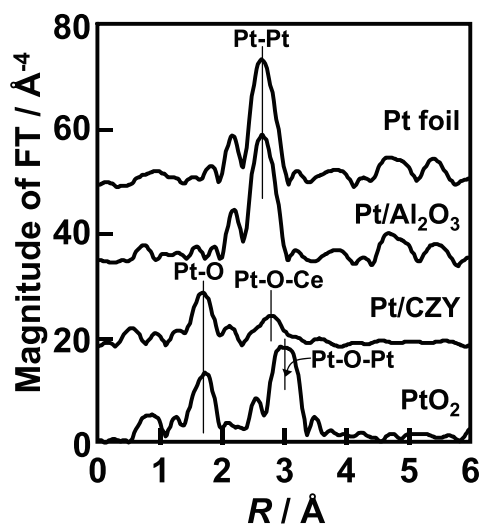
Fig. 7 Fourier-transforms of Pt L3-edge EXAFS spectra for supported catalysts after aged at 800°C in air and the standard samples of Pt foil and PtO 2 powder.
