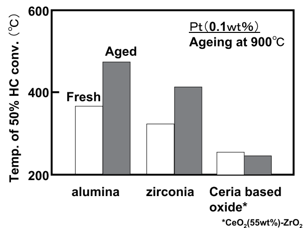
Fig. 13 Effect of support oxides for catalytic activities at 0.1 wt% Pt loading after aged at 900^\circ\text{C} in a simulated exhaust gas. (26)
