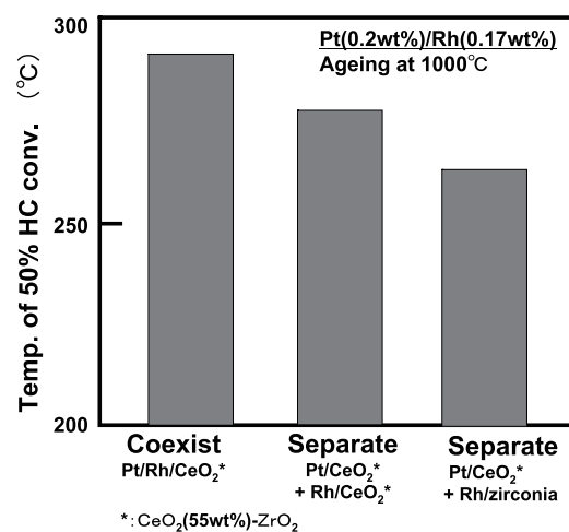
Fig. 14 Effect of configuration with 0.2 wt% Pt and 0.17 wt% Rh in catalysts for catalytic activities after aged at 1000^\circ\text{C} in a simulated exhaust gas. (26)
