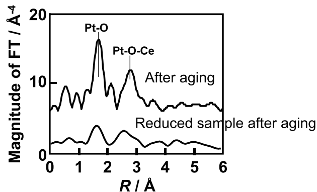
Fig. 8 Fourier-transforms of Pt L3-edge EXAFS spectra for the CZY catalysts after aged at 800°C in air and subsequent reduction treatment. (19)
