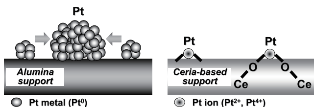
Fig. 9 Mechanism illustration of the Pt sintering inhibition on the conventional Pt/alumina and the Pt/ceria-based oxide.
