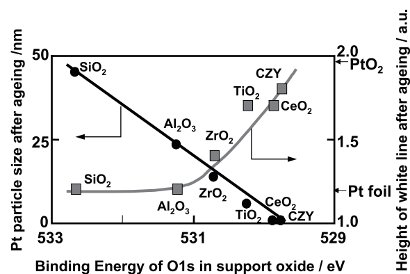
Fig. 10 Pt-oxide support interaction and correlation with Pt sintering in an oxidizing atmosphere. (19)
